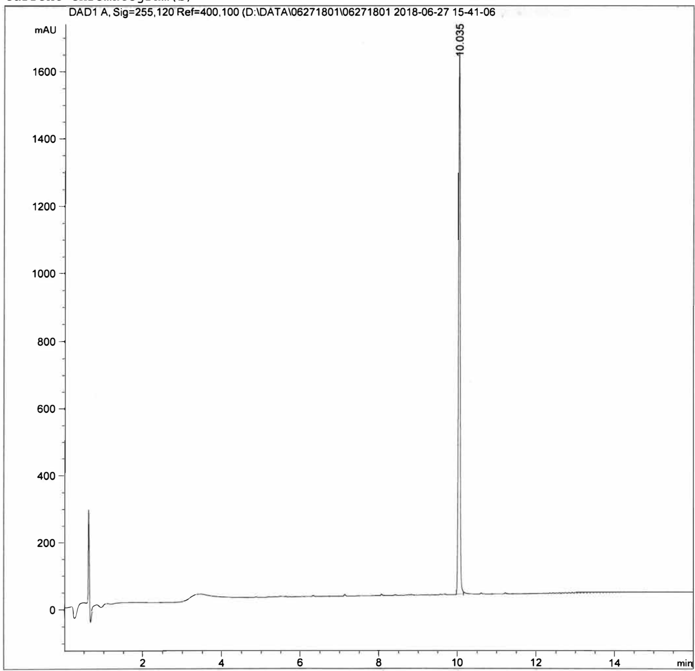
Current Chromatogram(s)
