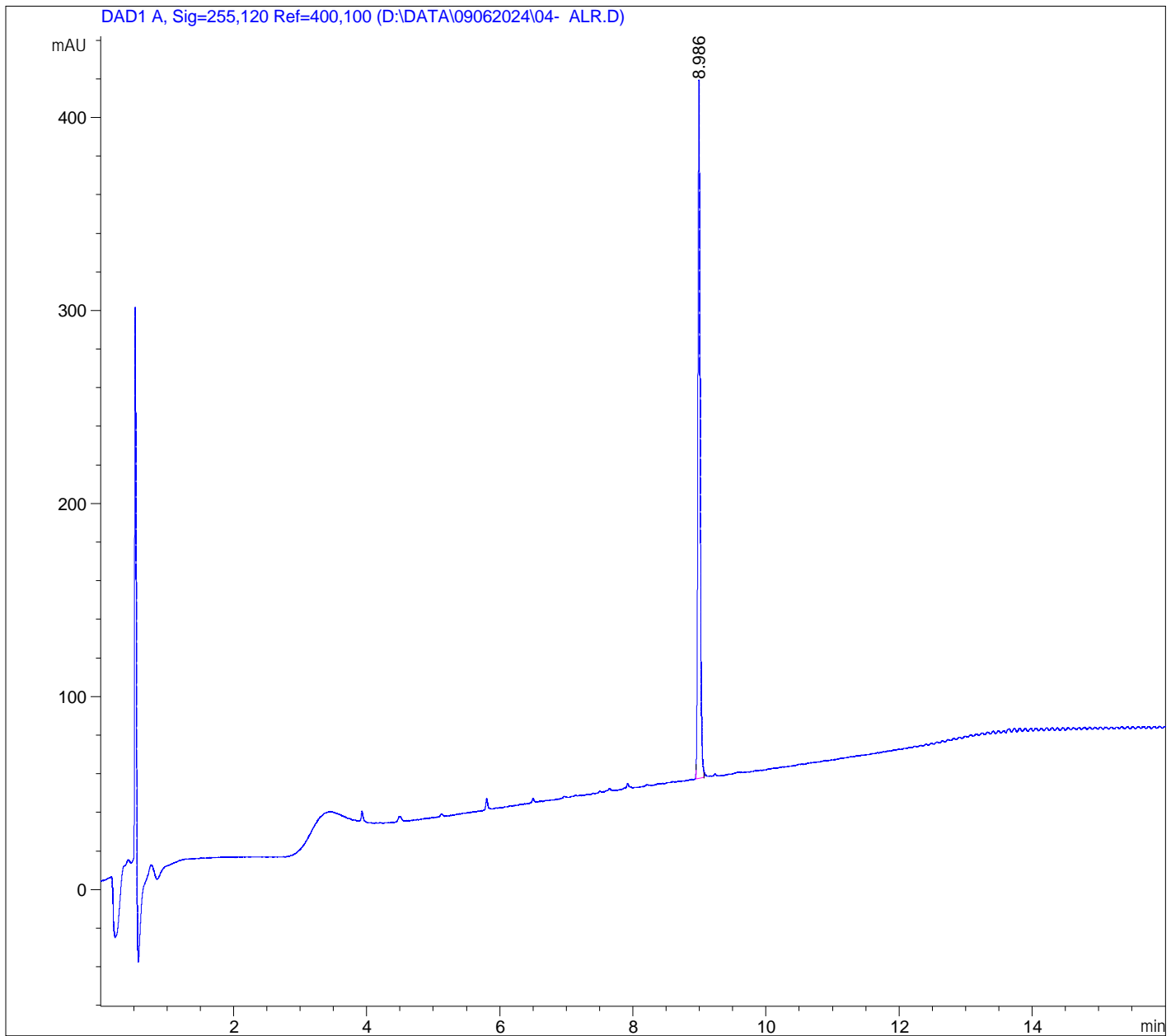
Current Chromatogram(s)
