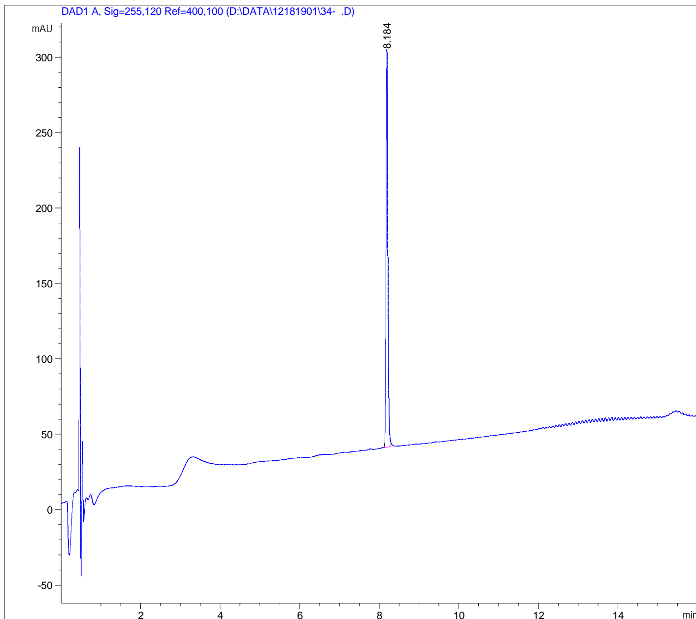
Current Chromatogram(s)
